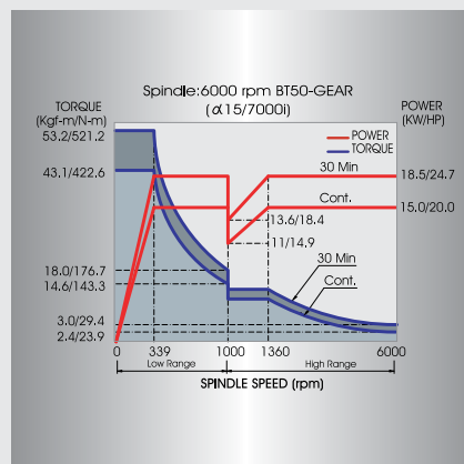
High Torque With Low And High Speed.
