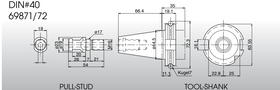
BT#50
