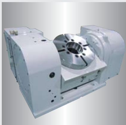
Tilting Rotating Table 200/350/450mm With Option Angle Encoder (A+C).
