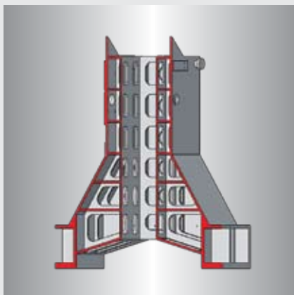
Double Rigidity Wide Column Without Counter Weight.
